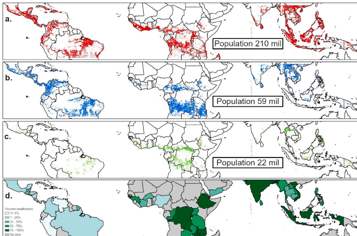
Fig. 2. Panels a-c: Tropical areas with tree cover restoration potential between 2020 and 2050 at an incentive of \$20 \text{ tCO}_2^{-1} following (Busch et al., 2019) and (Erbaugh et al., 2020), classified according to dominant land use: cropland based on (Fritz et al., 2015), (a), pastureland based on (Ramankutty et al., 2008), (b), and degraded forestland as the residual (c), with population size based on (CIESIN, 2018). Panel d: National percentages of smallholdings in agricultural land area, based on (Lowder et al., 2021).
