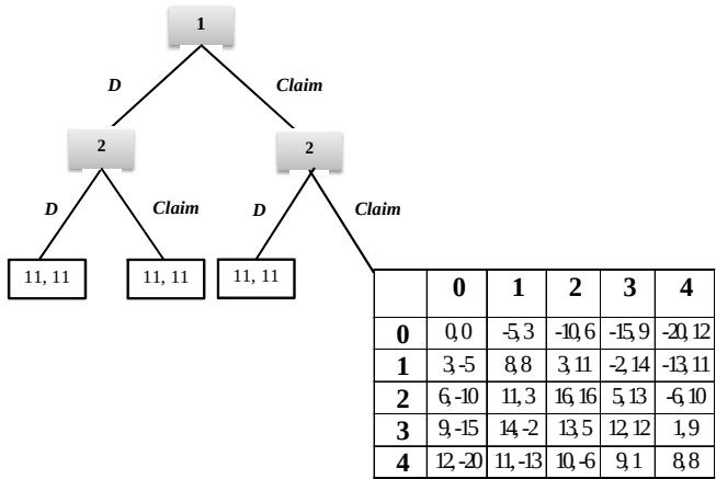
Figure 3. Divider Game
